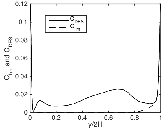
Figure 4.7: C_{DES} and C_{lim} value across channel at Ro = 1.5
