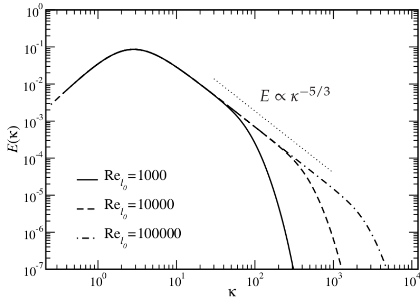
Figure 2.1: Energy spectrum for varying Reynolds number [Pope (2000)]
